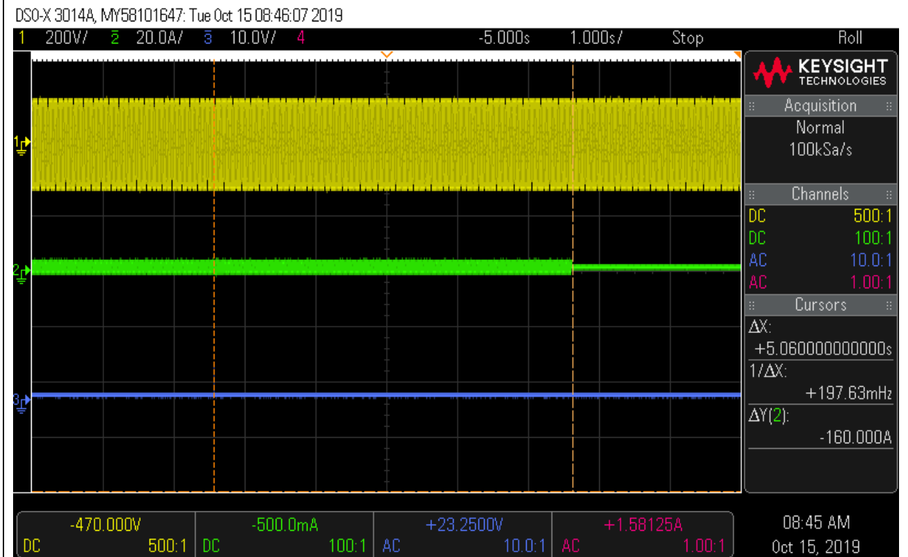
Trip time (5s setting)
