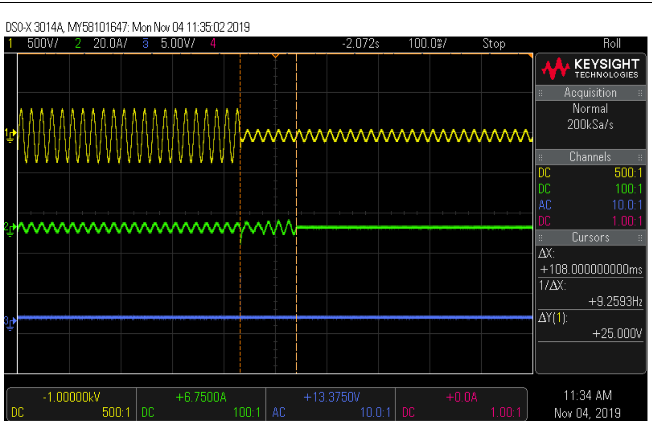
Trip time (0.1s setting)
