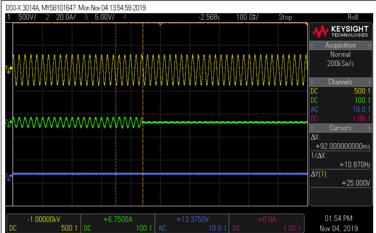
Trip time (0.1s setting)
