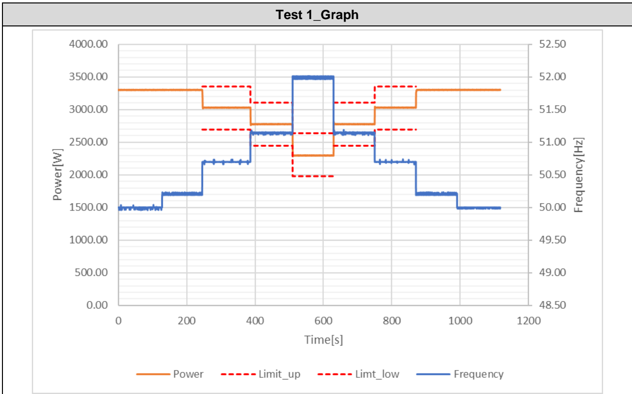
Intentional delay time (2s)
